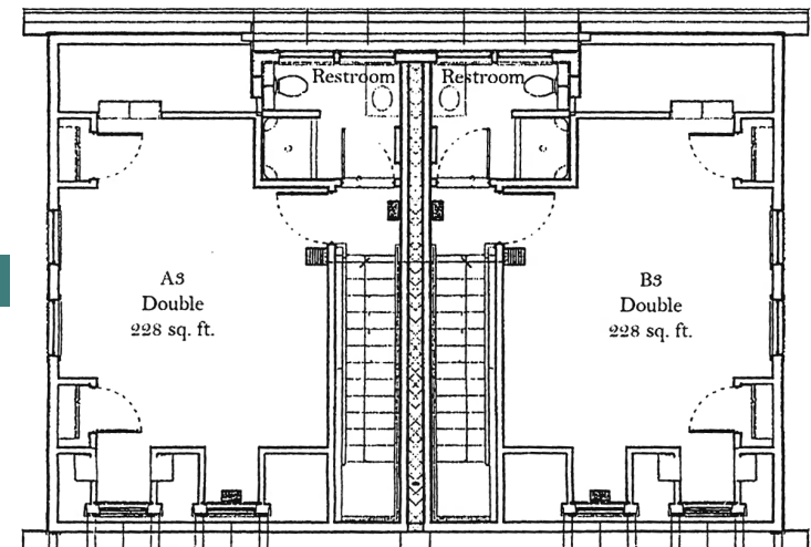
THIRD FLOOR
