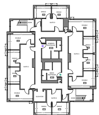
NINTH FLOOR
