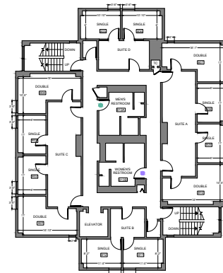
EIGHTH FLOOR
