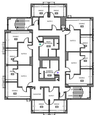
SIXTH FLOOR
